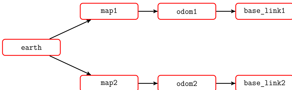
Figure 4.32: Arrangement of standard frames in ROS for a multiple robot application.
