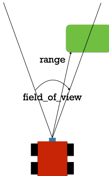
Figure 7.5: Meaning of the parameters included in a sensor_msgs::Range message.
